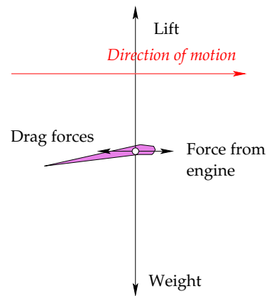
Figure 1.1. The forces on a steadily-flying plane. This figure shows the wing of the plane.
