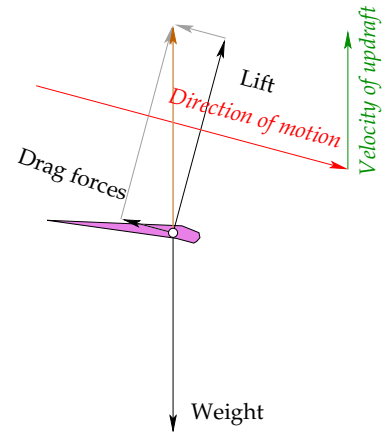
Figure 1.4. Add an updraft.
