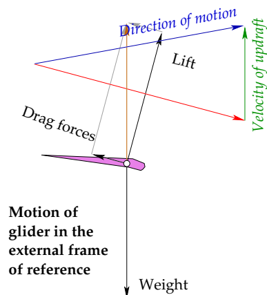
Figure 1.9. A recap of the glider in the updraft, from figure 1.5b.
