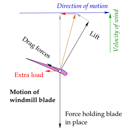
Figure 1.8. Top view of a wind turbine’s blade.
