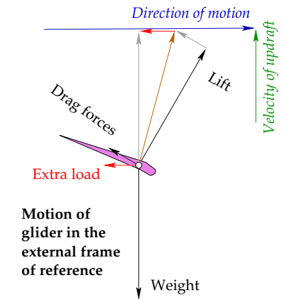
Figure 1.7. How the forces on the glider add up.
