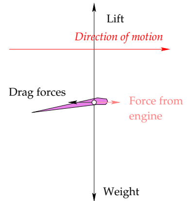
Figure 1.2. The forces on a plane when the engine is suddenly switched off.
